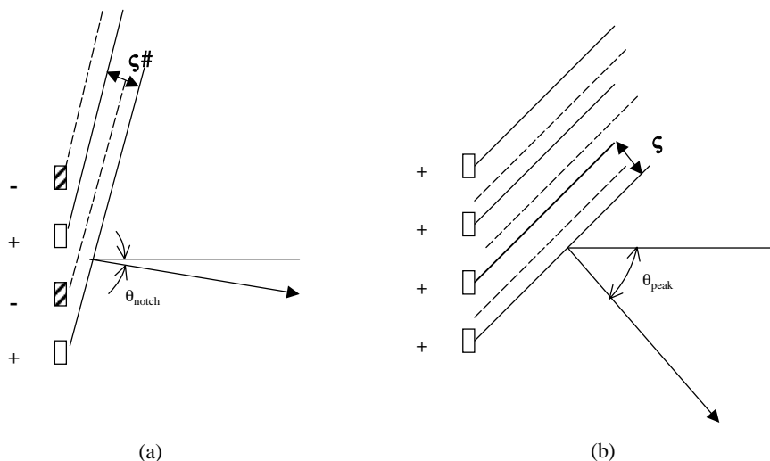
Fig. 7. For a distant observation point, Fresnel circles are transformed into segments. (a) When observing at angle \theta_{notch} , half the sources are in phase opposition with the other half, thus producing a null pressure. (b) As we move further off axis, all sources are in phase, thus producing a strong pressure.
