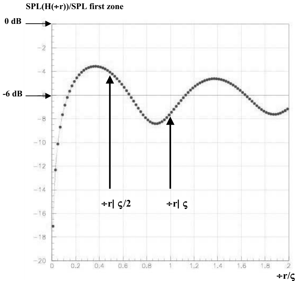
Fig. 26. Normalized SPL of segment H(\Delta r) , defined in Fig. 25, displayed as a function of increase in radius of circle.
