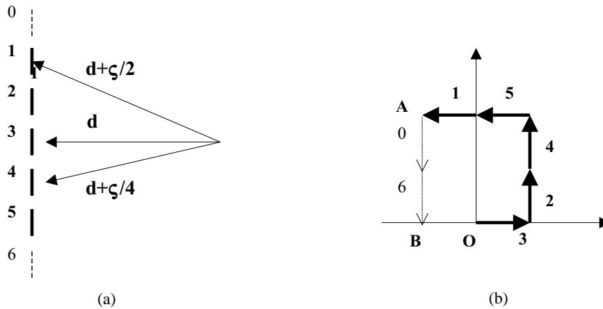
Fig. 24. (a) First Fresnel zone broken into 5 segments of equal sound pressure. (b) Argand diagram of complex amplitudes associated with these segments and their resultant sum.
