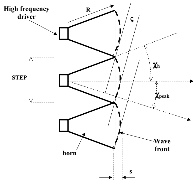
Fig. 8. Vertically arraying conventional horns will not produce a flat wavefront. \theta_h is defined as half the vertical coverage angle for the individual horn, the listener position is at infinity, and the Fresnel circles become straight lines that are tangential to each individual horn wavefront at location \theta_{peak} . This angle \theta_{peak} corresponds to a peak in SPL when the Fresnel ring spacing is \lambda .
