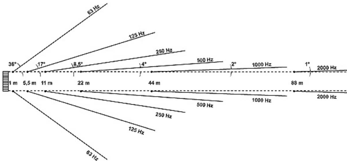
Fig. 2. Variation of border distance and far-field coverage angle with frequency for a flat line source array of 5.4-m height.
