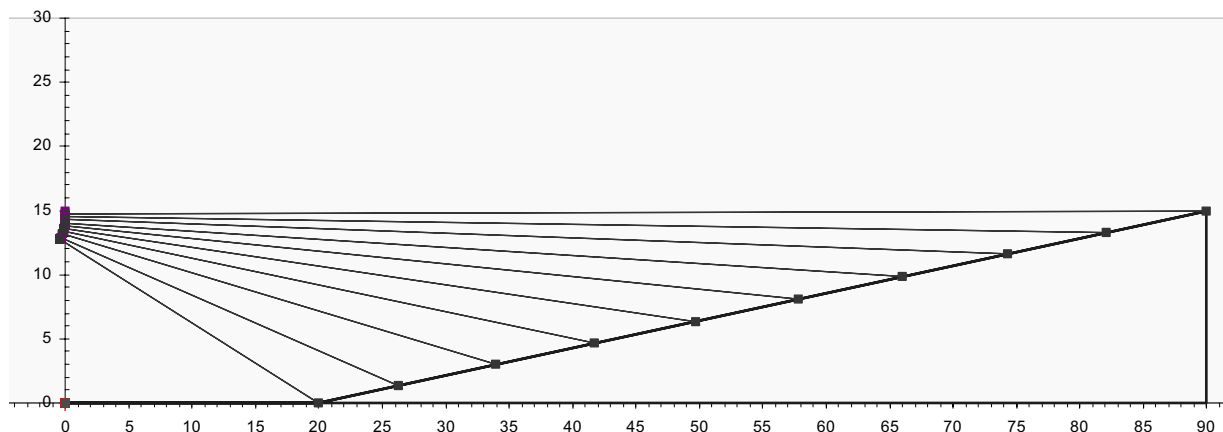
Fig. 21. Wavefront sculpture where a variable-curvature line array is designed so that \alpha d = \text{constant} over audience geometry.
