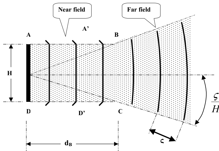
Fig. 1. Radiated SPL for line source AD of height H . In the near field, SPL decreases as 3 dB per doubling of distance whereas in the far field, SPL decreases as 6 dB per doubling of distance.
