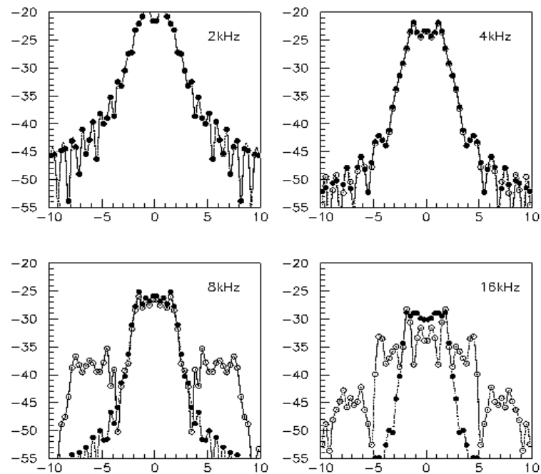
Fig. 10. SPL along a vertical path, 20 m away from vertical array of 30 horns (total height = 4.5 m, wavefront curvature S = 10 mm) calculated at 2, 4, 8, and 16 kHz. ○ Line array; ● continuous line source.
