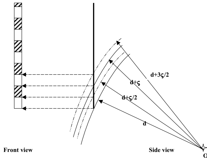
Fig. 4. Observer O is no longer on axis to line source and corresponding Fresnel zones for an off-axis observer O (front view). There is no dominant zone, and individual zones cancel each other.
