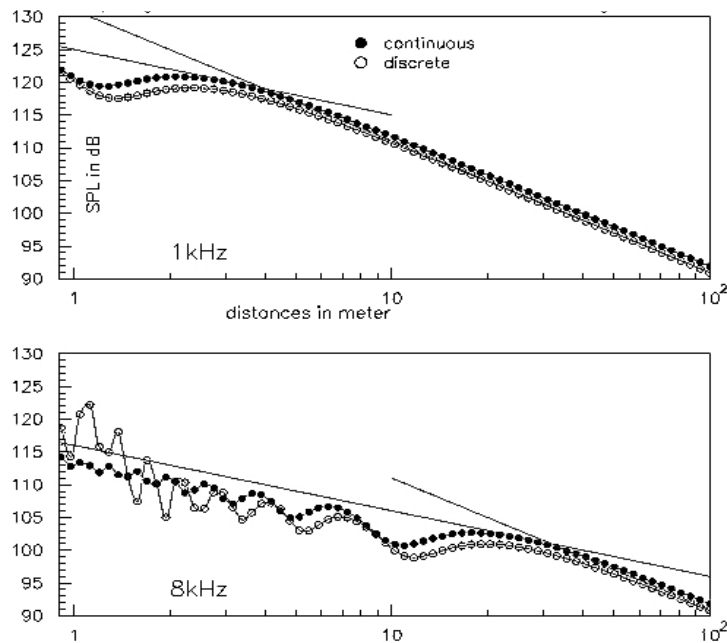
Fig. 12. SPL as a function of distance. \circ 23 tweeters totaling a height of 1.76 m; \bullet continuous array of same height. The -3 dB and -6 dB per doubling of distance lines are shown to indicate the border between near and far fields.
