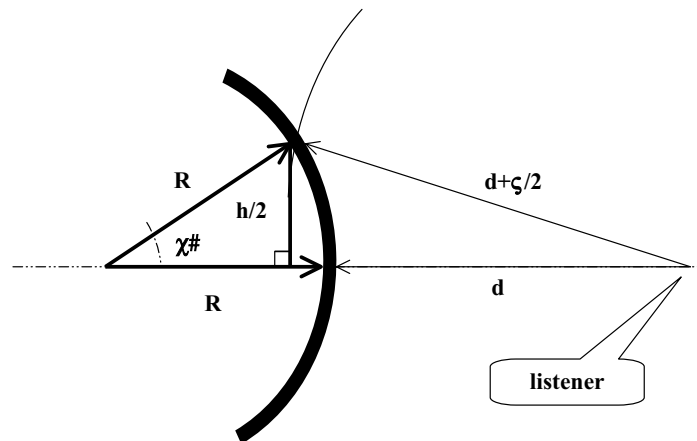
Fig. 20. Nomenclature for calculating the size of the first Fresnel zone for a curved array.
