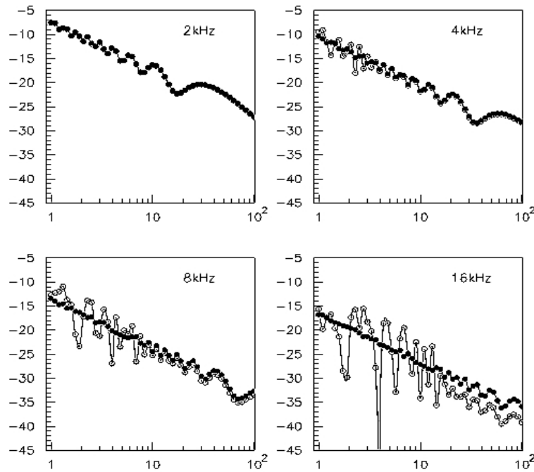
Fig. 9. SPL versus distance for vertical array of 30 horns (total height = 4.5 m, wavefront curvature S = 10 mm) calculated at 2, 4, 8, and 16 kHz. ○ Line array; ● continuous line source.
