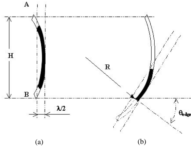
Fig. 17. (a) Curved array AB with the first Fresnel zone shown in black for a distant on-axis observation point. (b) At angle \theta_{edge} the size of the first Fresnel zone is half the size on axis, corresponding to a 6-dB reduction in SPL and defining the vertical directivity of the curved array.
