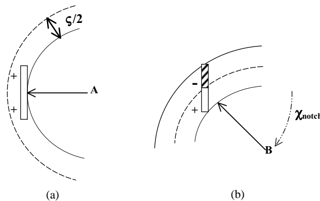
Fig. 13. (a) First Fresnel zone is larger than height of array; entire array is in phase. (b) When rotating around the array there may be an angle where one-half the array is in phase opposition to the other half.
