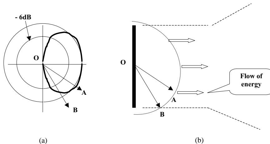
Fig. 23. (a) Polar diagram where flow of energy is supposed to emanate from point source O (along OA, for instance). (b) Using such a polar diagram in the near field would be incorrect for characterizing a line source.
