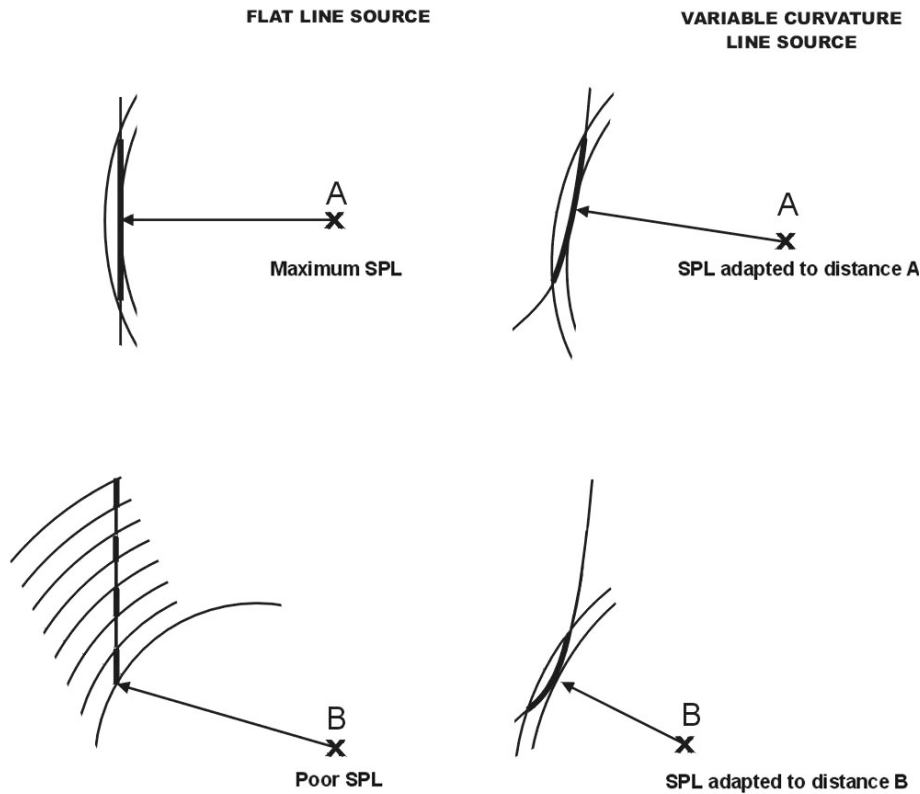
Fig. 19. Comparison of flat and variable-curvature arrays. SPL distribution of the variable-curvature array is adapted to suit the audience geometry.
