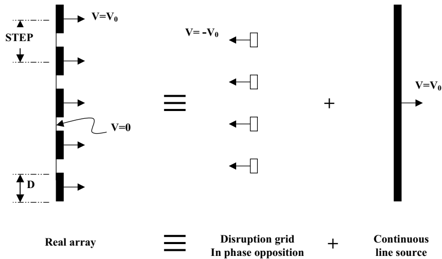
Fig. 6. A real array consisting of sources of size D spaced apart by distance STEP (left) can be considered as equivalent to the sum of a disruption grid and a continuous ideal source (right).
