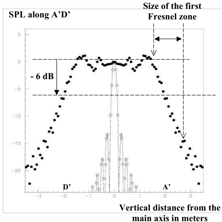
Fig. 15. ● SPL along A'D' (see Fig. 1) for a line source ( H = 4 m) at a distance of 9 m, for F = 4 kHz; ○ SPL calculated incorrectly using analytical expression for far-field directivity of same line source.
