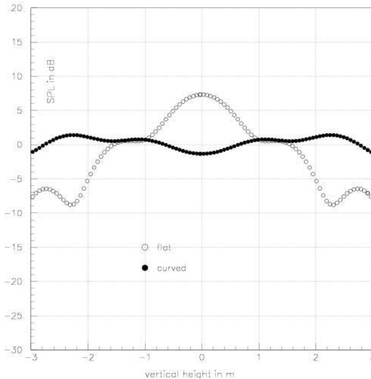
Fig. 18. Comparison of flat and curved line source arrays of the same height. SPL is calculated along a vertical line 20 m from the sources. The curved line source presents less variation in its vertical SPL pattern but with reduced on-axis SPL.
