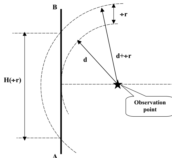
Fig. 25. Circle of radius d drawn from the observation point, tangent to line source AB. Drawing a circle of radius (d + \Delta r) defines a segment of height H on AB.
