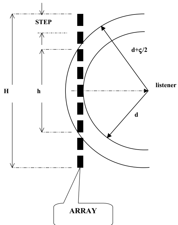
Fig. 11. First Fresnel zone height is h . This height grows as distance d increases until h = H . At greater distances, no more increase of radiated power is expected.
