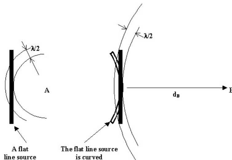
Fig. 16. At position A, wave field of flat line source is cylindrical. At position B, the border between near and far fields has been reached. By curving the array, the border distance is further away than position B since the entire curved line source is not entirely contained within the first Fresnel zone.
